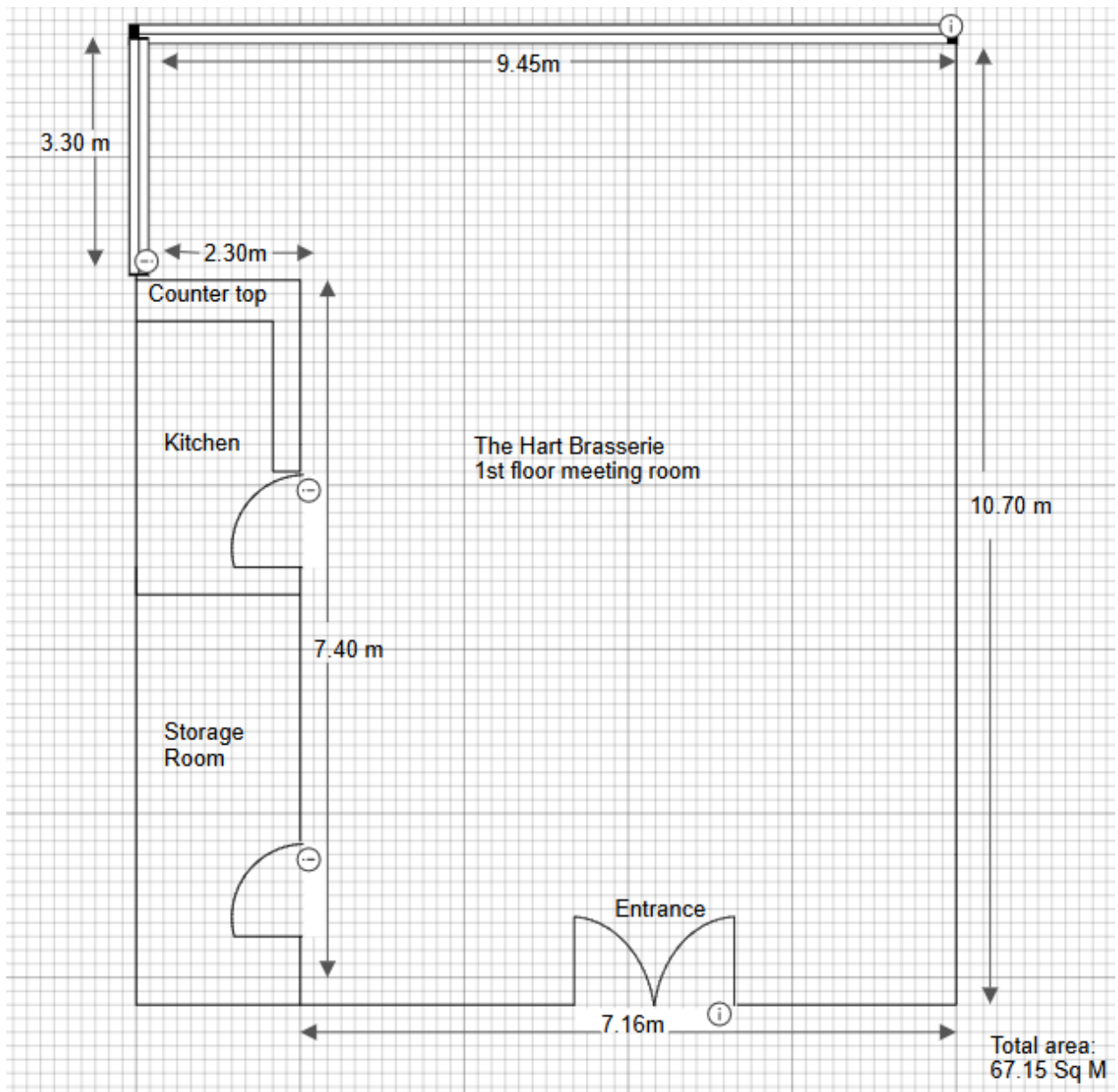
The Hart Brasserie – 1 st floor meeting room floor plan
